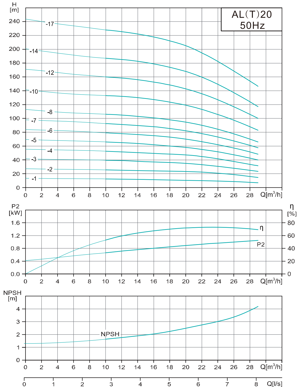
Performance Curve of AL(T)20
